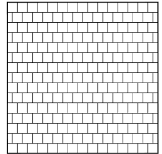
Pattern OM.9. Half Block Stretcher Course 100 No. Half Block 100x100mm per sq.m.
