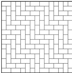
Pattern OM.5. Double Herringbone 50 No. Omega 200x100mm per sq.m.
