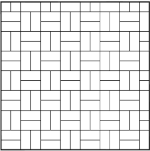
Pattern OM.4. Basket Weave 50 No. Omega 200x100mm per sq.m. *Not recommended for driveways
