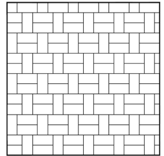
Pattern OM.6. Mixed Stretcher Course 50 No. Omega 200x100mm per sq.m.
